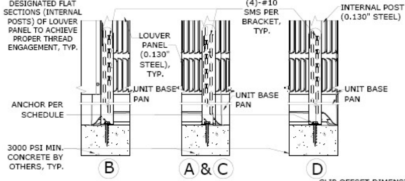
3 TIE-DOWN BRACKETS N.T.S. ELEVATION
