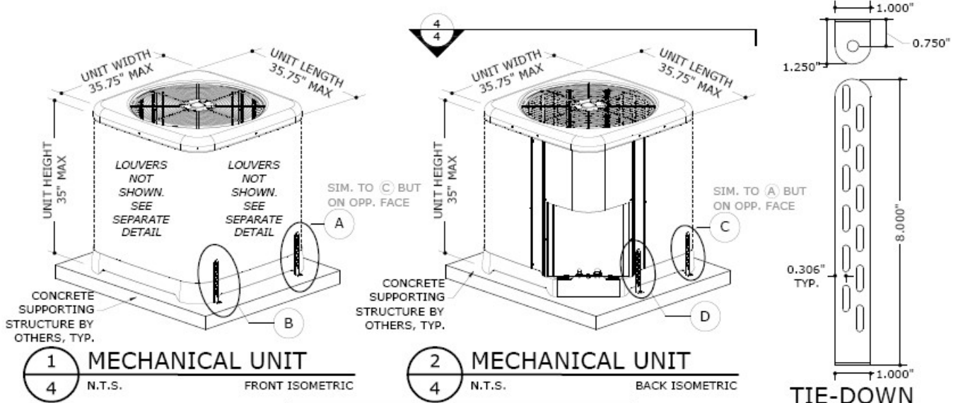
TIE-DOWN BRACKET MIAMI TECH CLIP: 14GA (0.07") ASTM A653 Fy=33 KSI STEEL (CUTD8) OR 0.080" 5052-H32 ALUMINUM (CUTD8), MIAMI TECH KIT # TZFCUTDSMK OR TZFCUTDASMK
