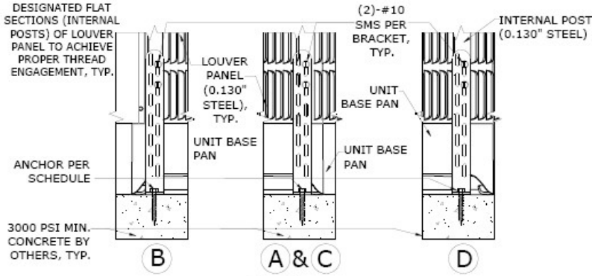
3 TIE-DOWN BRACKETS N.T.S. ELEVATION
