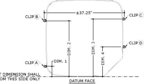
4 TIE-DOWN BRACKET LAYOUT N.T.S. PLAN
