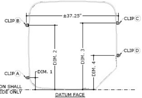
4 TIE-DOWN BRACKET LAYOUT N.T.S. PLAN
